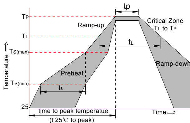
FIG.2: Reflow condition
